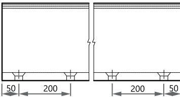
Drilling for profil 1500 mm
