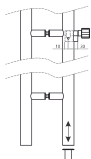
half- profile cylinder 30/10 with knob
