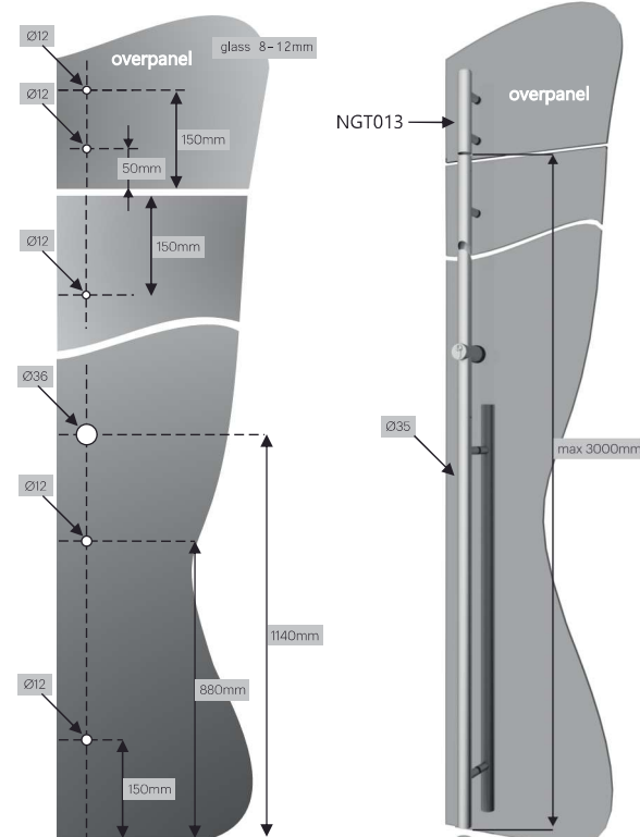
NGT013 bush screwed to overpanel through glass drilling
