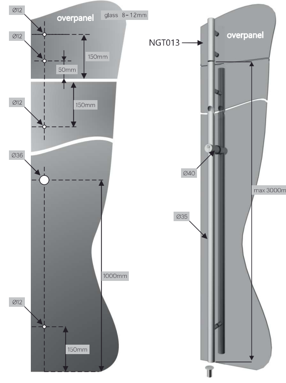
NGT013 bush screwed to overpanel through glass drilling
