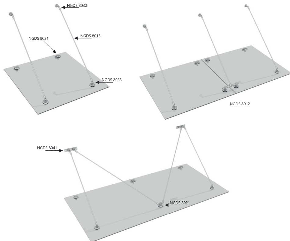
an example mount on the wall with insulation
