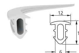
NGDU 06 joint gab compression profile
