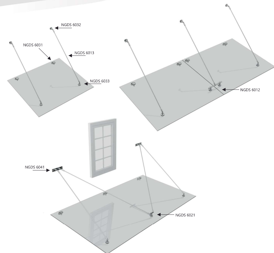
an example mount on the wall with insulation
