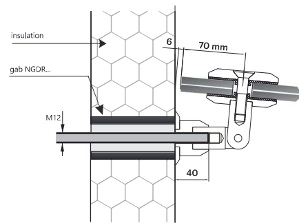
an example mount on the wall with insulation
