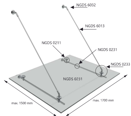
NGDS 6032 wall mount-connection
