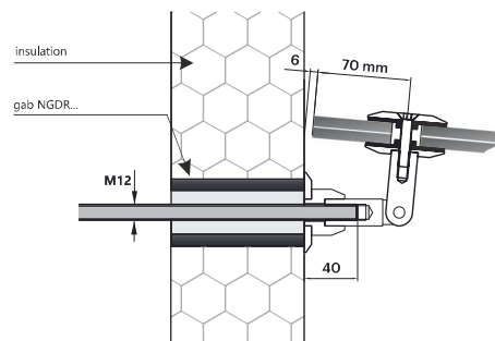
an example mount on the wall with insulation
