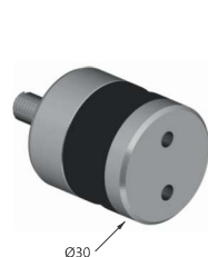
pts.20.01 glass point fittings glass drilling \varnothing 16
